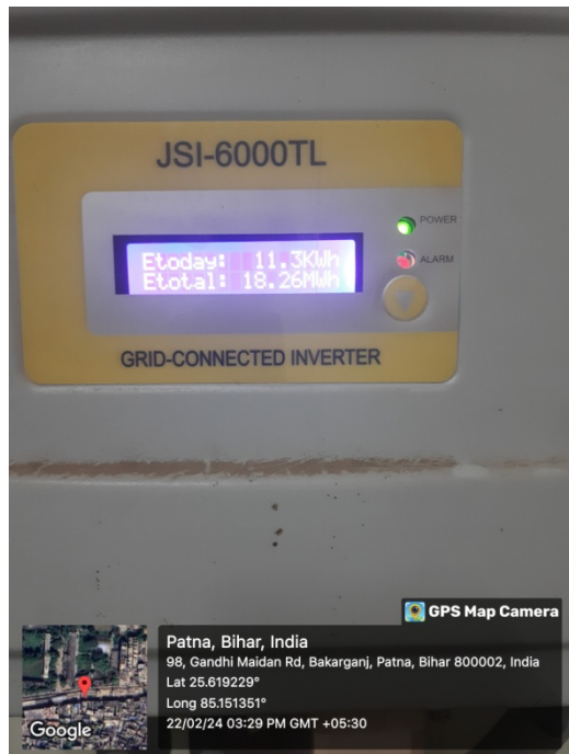
Inverter and AC & DC box of solar power plant
